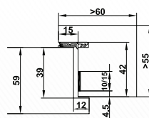
CombiModul-Blockrahmen
