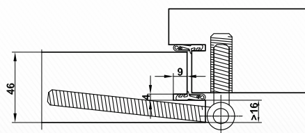
CompactWinTop 46mm
