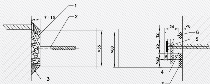
Wandanschlüsse
