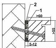
Blockrahmen MBW CombiModul
