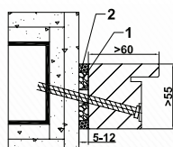
Blockrahmen LBW CombiModul
